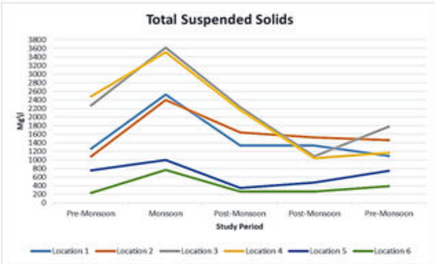
Figure 10: Variation in Total Suspended Solids
