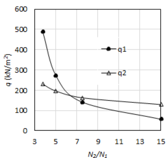
Fig. 6.2 N_2/N_1 Vs q_1 and q_2 for D/d=2.5 and N_1=15
