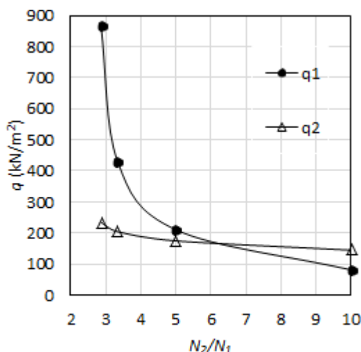
Fig. 5.1 N_2/N_1 Vs q_1 and q_2 for D/d=2.0 and N_2=10
