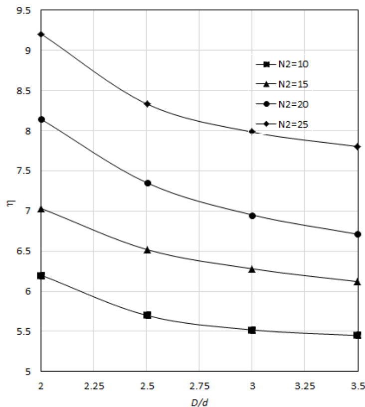
Fig. 9 D/d Vs \eta for Equalization of Ultimate Bearing Capacity, q_1 = q_2
