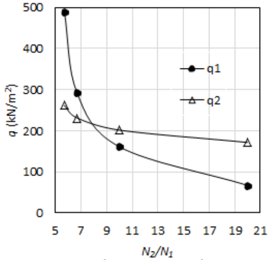
Fig. 7.1 N_2/N_1 Vs q_1 and q_2 for D/d = 2.0 and N_1 = 20
