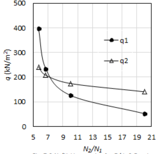
Fig. 7.2 N_2/N_1 Vs q_1 and q_2 for D/d = 2.5 and N_1 = 20
