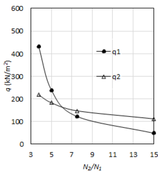
Fig. 6.3 N_2/N_1 Vs q_1 and q_2 for D/d = 3.0 and N_1 = 15
