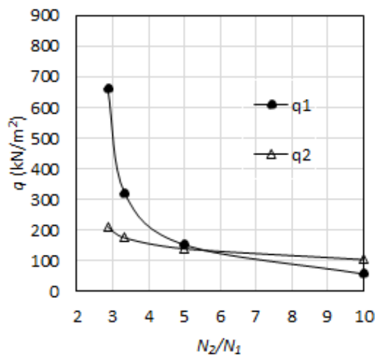
Fig.5.3 N_2/N_1 Vs q_1 and q_2 for D/d=3.0 and N_1=10
