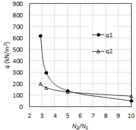
Fig.5.4 N_2/N_1 Vs q_1 and q_2 for D/d=3.5 and N_1=10
