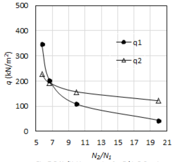
Fig. 7.3 N_2/N_1 Vs q_1 and q_2 for D/d = 3.0 and N_1 = 20
