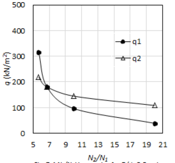
Fig. 7.4 N_2/N_1 Vs q_1 and q_2 for D/d = 3.5 and N_1 = 20
