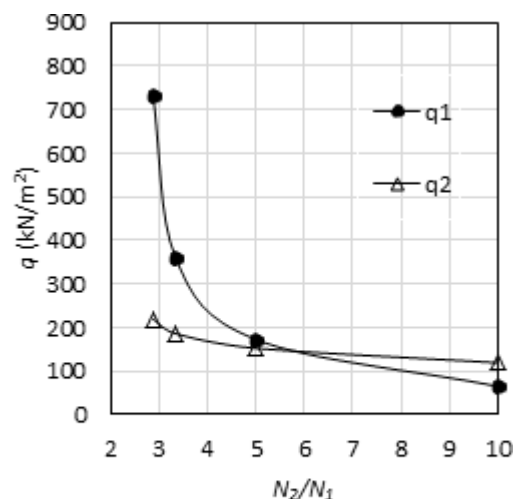
Fig. 5.2 N_2/N_1 Vs q_1 and q_2 for D/d=2.5 and N_2=10
