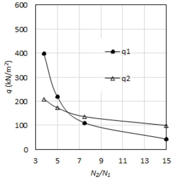
Fig. 6.4 N_2/N_1 Vs q_1 and q_2 for D/d = 3.5 and N_1 = 15
