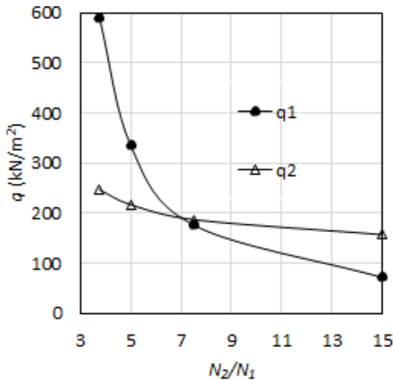
Fig. 6.1 N_2/N_1 Vs q_1 and q_2 for D/d=2.0 and N_1=15
